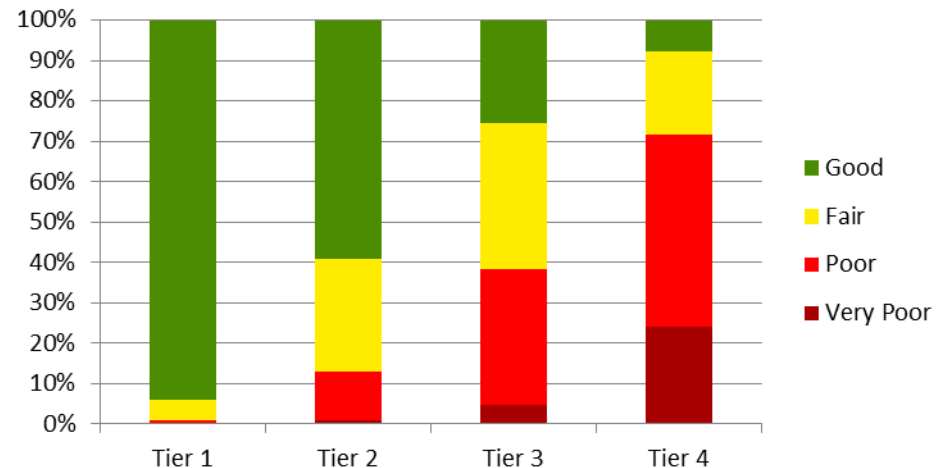
Condition of Pavements by Tier (miles)
